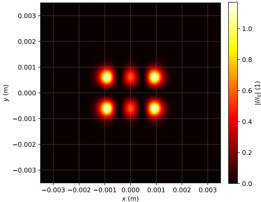
Intensity profile I(x, y, z = 1.194)/I_0 , P_{in}=2.0P_{cr} , artificial time
